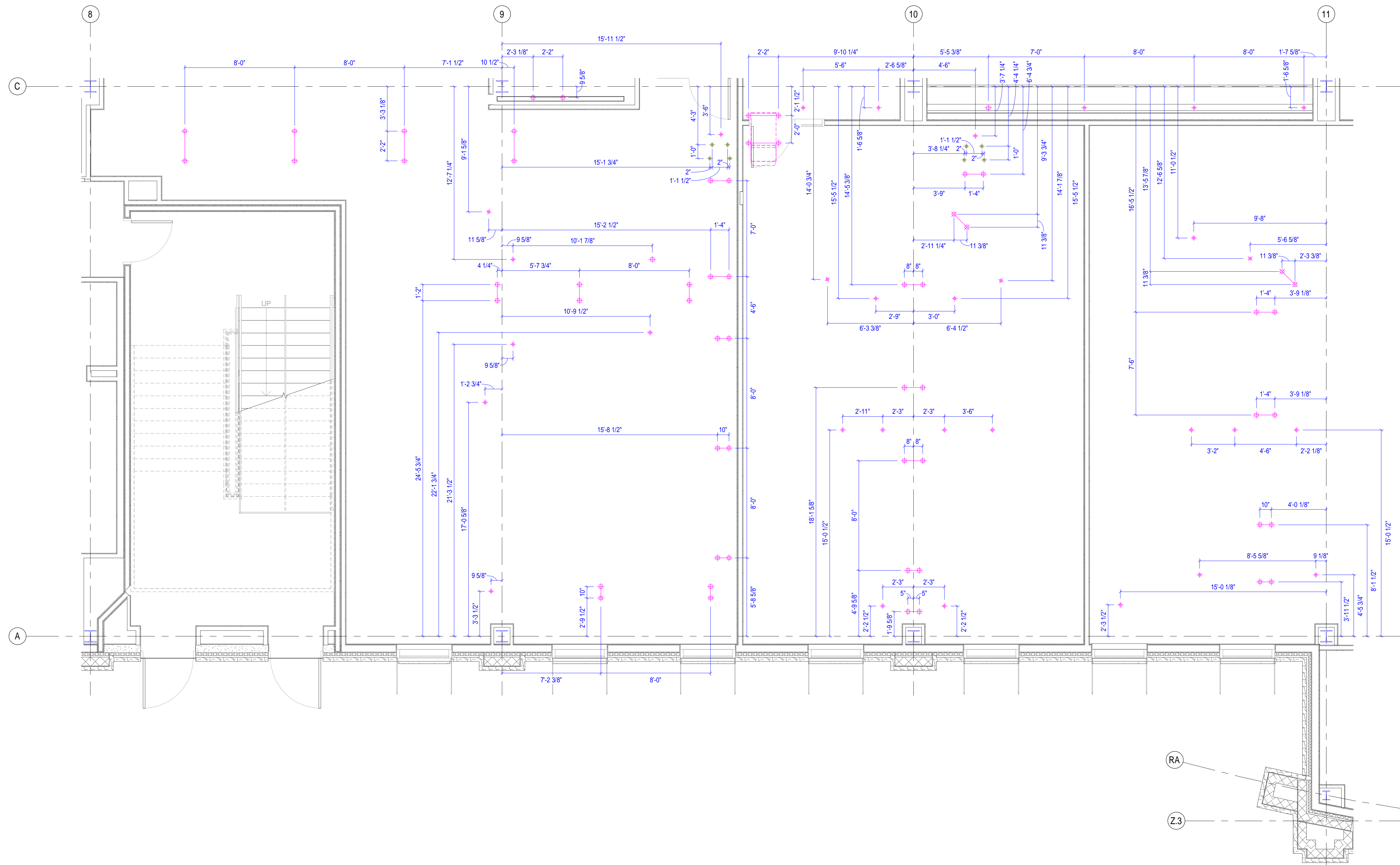
FIRST FLOOR PLAN - PART 6 - HVAC HANGERS
